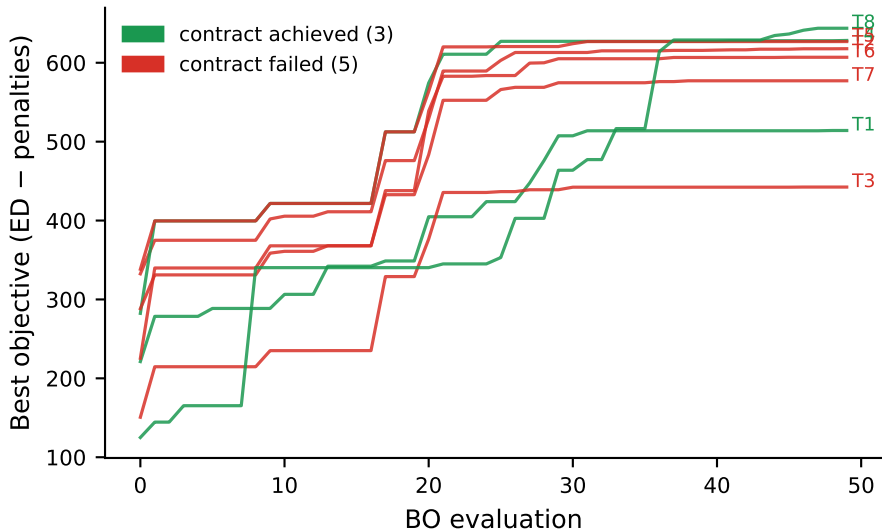
Bayesian optimization trajectories (Ax, seed 1234, 50 evals)
