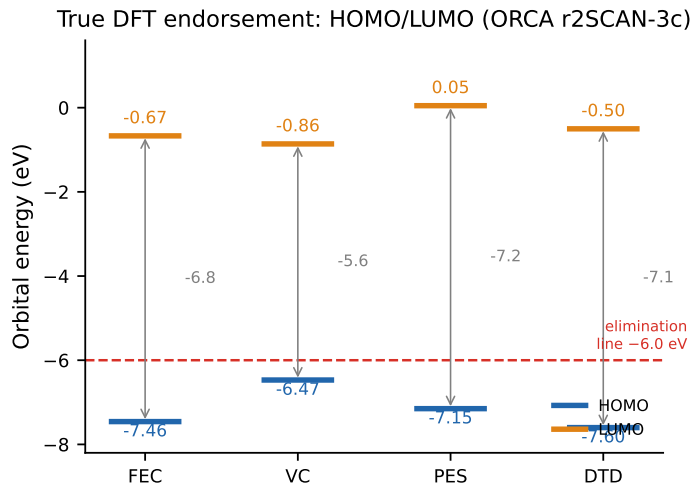
Figure 10: HOMO/LUMO levels of the four funnel-passed molecules at the r2SCAN-3c level (ORCA), against the funnel’s -6.0 eV oxidation-stability elimination line. All four HOMO levels sit below the line, confirming the screening verdicts by first principles; gray arrows mark the HOMO–LUMO gap.
