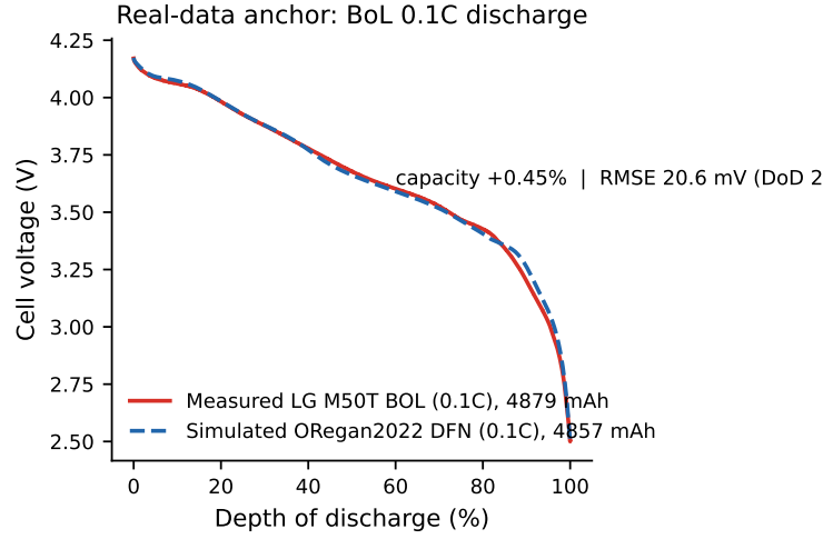
Figure 6: Real-data anchor: beginning-of-life 0.1C discharge of a production LG M50T 21700 cell (Imperial College dataset, [21]) versus the ORegan2022-parameterized DFN simulation [23]. Capacity agrees to +0.45%; voltage RMSE 20.6 mV over 2–82% depth of discharge.
