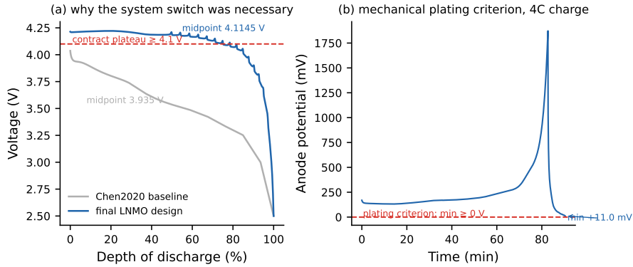
Figure 12: The T6 case at curve level. (a) 1C discharge: the Chen2020 baseline’s midpoint voltage sits below the 4.1 V contract plateau, which is what the ceiling assessment diagnosed; the final LNMO design clears it (4.1145 V). (b) The final design’s anode potential during 4C charge stays above the 0 V plating criterion throughout (min +11.0 mV).
