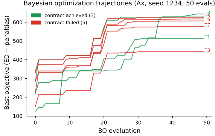
Figure 6: Bayesian optimization best-objective trajectories per task (Ax, Sobol initialization, GPEI + LogNEI, seed 1234, 50 evaluations). The three structural tasks (T1/T4/T8) achieve their contracts; the five material-bottleneck tasks plateau against penalties (plating, SEI, plateau, nail) that no structural parameter can remove.
