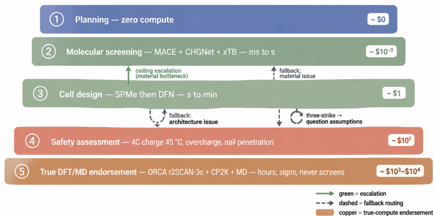
Figure 3: The multi-precision funnel: cost rises from planning (zero compute) to true DFT/MD endorsement (hours), which signs conclusions and never screens. Fallback routes a failure to the scale of its cause; ceiling escalation opens the material lever when the cell-scale ceiling cannot close the gap.
