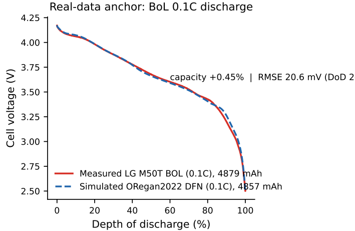
Figure 4: Real-data anchor: beginning-of-life 0.1C discharge of a production LG M50T 21700 cell (Imperial College dataset, [7]) versus the ORegan2022-parameterized DFN simulation [9]. Capacity agrees to +0.45%; voltage RMSE 20.6 mV over 2–82% depth of discharge.
