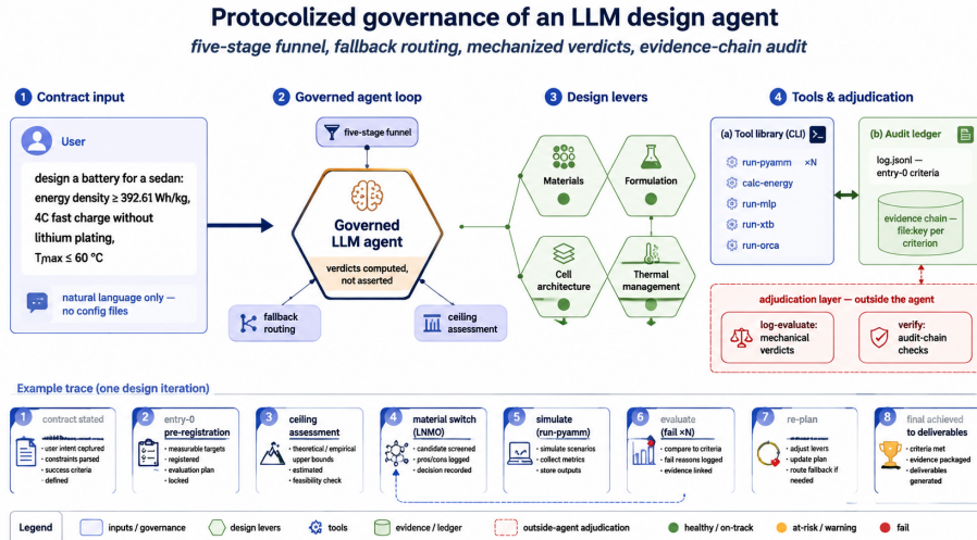
Figure 2: System architecture. The natural-language contract is the sole input; the agent executes the five-stage loop over a command-line tool library; the adjudication layer sits outside the agent and writes mechanized verdicts with per-criterion evidence into the audit ledger.
