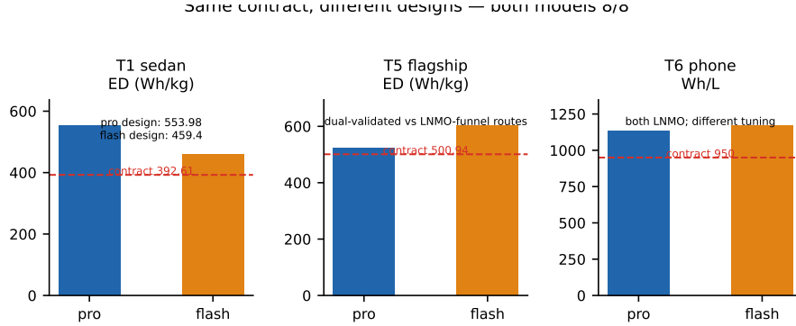
Figure 10: Model robustness with design diversity: the same contracts attained under both models with different designs (T1: 553.98 vs 459.4 Wh/kg; T5: 524.2 vs 603.6; T6: 1135.8 vs 1172.1 Wh/L). Contract attainment is reproducible; the solution space stays broad.
