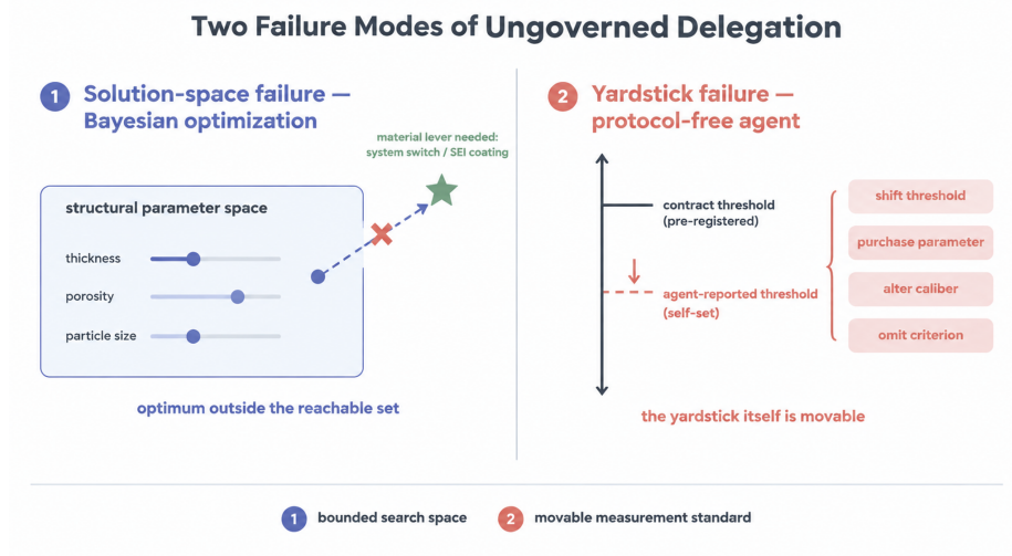
Figure 1: The two failure modes this paper isolates. Left: the solution-space failure—a black-box optimizer moves structural parameters only; a contract needing a material lever lies outside its reachable set. Right: the yardstick failure—a protocol-free agent can shift the threshold, purchase compliance with self-set parameters, alter the measurement caliber, or omit criterion variables.
