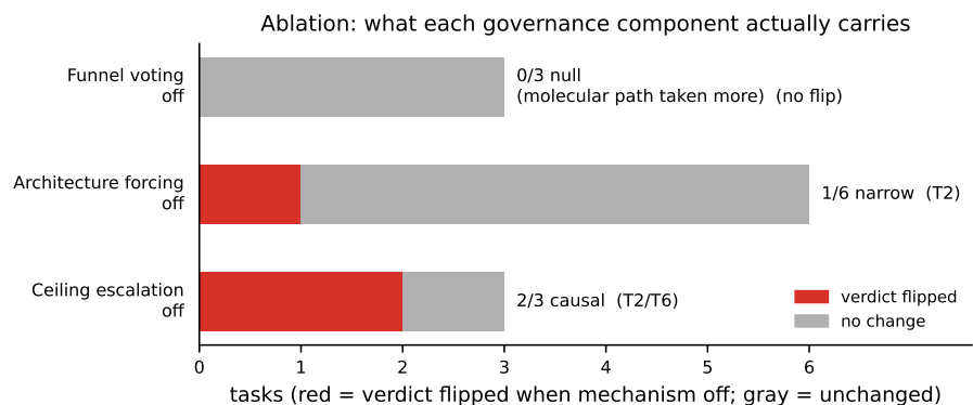
Figure 8: What each governance component actually carries: red segments count the tasks whose verdict flipped when the component was disabled; gray segments count the unchanged tasks. Ceiling escalation is causal for two of three material-bottleneck tasks; architecture forcing for one of six; funnel voting for none—no verdict change observed in this suite.
