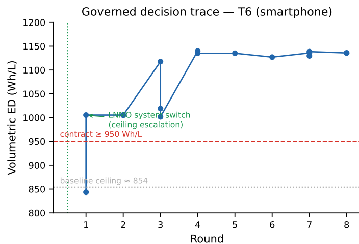
Figure 9: Governed decision trace on T6 (smartphone contract): volumetric energy density by round, with the contract line (950 Wh/L) and the baseline ceiling (854 Wh/L). The jump across the dashed line is the ceiling escalation—the LNMO system switch—followed by rounds of refinement to 1135.8 Wh/L.
