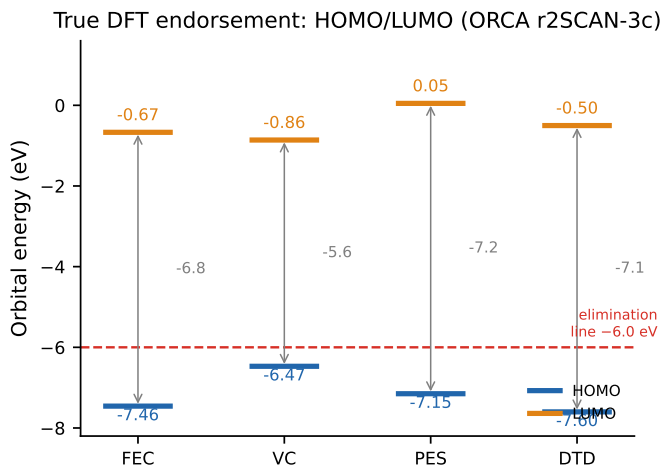
Figure 13: HOMO/LUMO levels of the four funnel-passed molecules at the r2SCAN-3c level (ORCA), against the funnel’s -6.0 eV oxidation-stability elimination line. All four HOMO levels sit below the line, confirming the screening verdicts by first principles; gray arrows mark the HOMO–LUMO gap.
