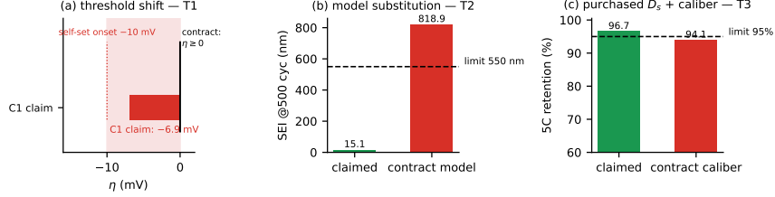
Figure 9: The yardstick failure modes of the protocol-free agent, re-adjudicated at the contract caliber: (a) threshold shift: T1’s -6.9 mV declared safe against a self-set -10 mV onset where the contract is zero tolerance; (b) model substitution: T2’s SEI claimed at 15.1 nm (500 cycles) under the solvent-diffusion-limited growth law, 818.9 nm under the contract’s ec-reaction-limited model with the full declared design; (c) purchased parameter plus caliber shift: T3’s 96.7\% retention against C/3 versus 94.1\% at the contractual 5C/1C with its declared diffusivities ( 84.8\% with standard ones).
