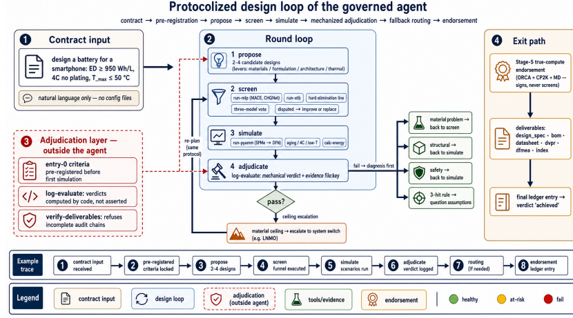
Figure 3: The protocolized design loop. The contract is the sole input; each round proposes, screens (when the bottleneck is molecular), simulates, and is adjudicated by code outside the agent; diagnosed failures route back to the scale of their cause, and a material ceiling escalates to a system switch. The red-dashed adjudication layer delivers the mechanical verdict and refuses incomplete audit chains; the exit path ends in endorsement and the deliverable package.
