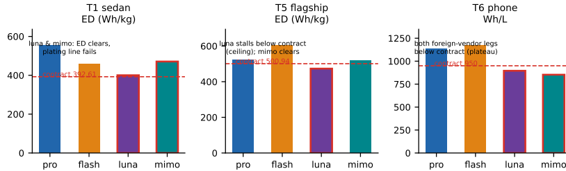
Figure 8: Model robustness with design diversity: the same contracts attained under the four models with different designs (T1: 553.98 vs 459.4 Wh/kg and a plating failure on both foreign-vendor legs; T5: 524.2 vs 603.6 vs 517.8). Red bar outlines mark legs that did not attain the contract (Table 3). Contract attainment is reproducible; the solution space stays broad.
