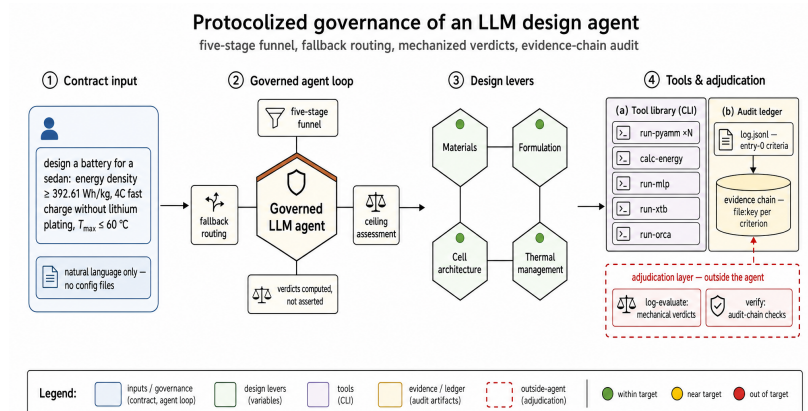
Figure 2: System architecture. The natural-language contract is the sole input; the agent executes the five-stage loop over a command-line tool library; the adjudication layer sits outside the agent and writes mechanical verdicts with per-criterion evidence into the audit ledger.
