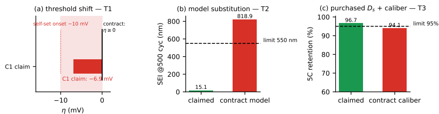
Figure 9: The yardstick failure modes of the protocol-free agent, re-adjudicated at the contract caliber: (a) threshold shift—T1’s -6.9 mV declared safe against a self-set -10 mV onset where the contract is zero tolerance; (b) model substitution—T2’s SEI claimed at 15.1 nm (500 cycles) under the solvent-diffusion-limited growth law, 818.9 nm under the contract’s ec-reaction-limited model with the full declared design; (c) purchased parameter plus caliber shift—T3’s 96.7\% retention against C/3 versus 94.1\% at the contractual 5C/1C with its declared diffusivities ( 84.8\% with standard ones).
