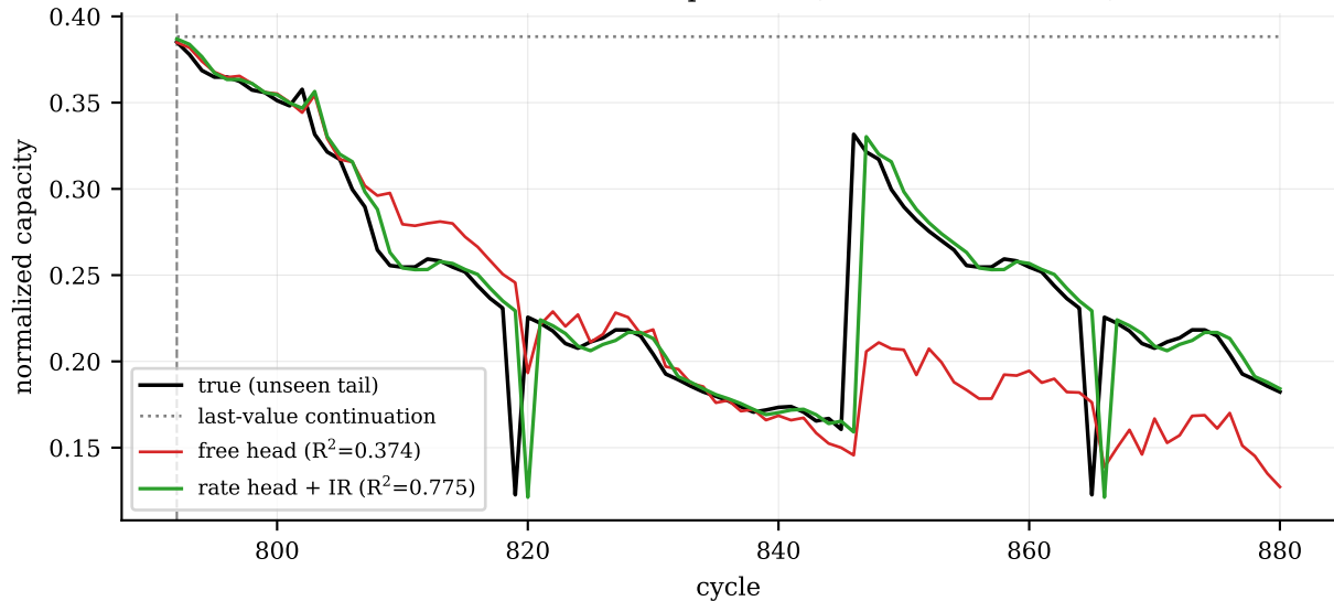
CALCE unseen-tail extrapolation (train 90%, eval 10%)
