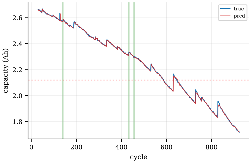
PANASONIC test cell
