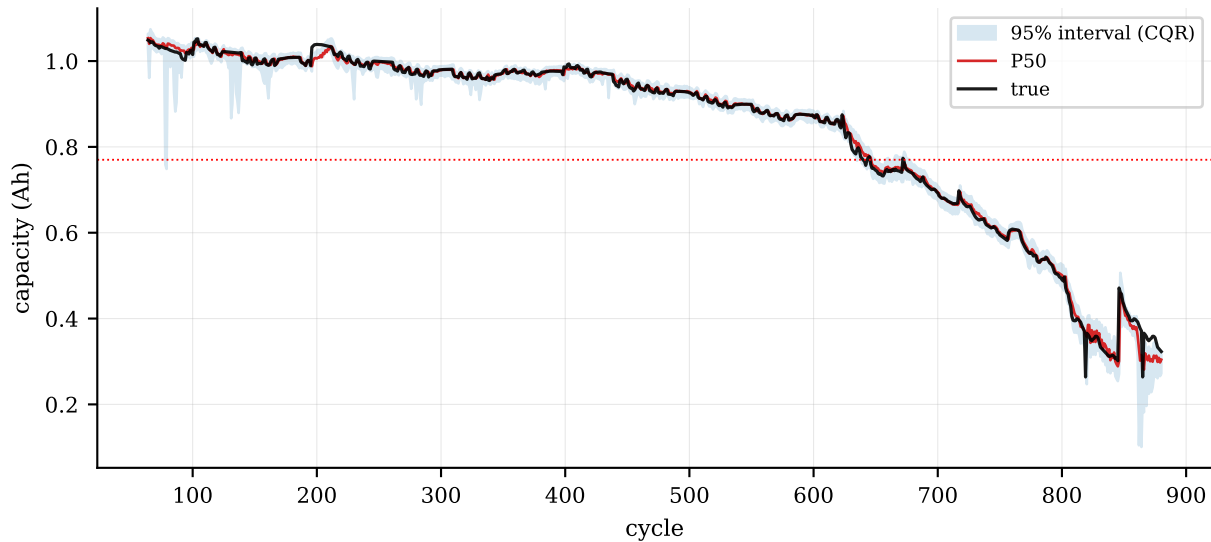
CALCE test cell: CQR-calibrated interval
