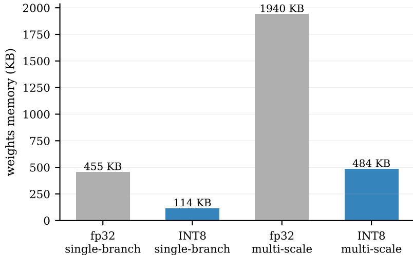
INT8 quantization: -75% memory, lossless AE
