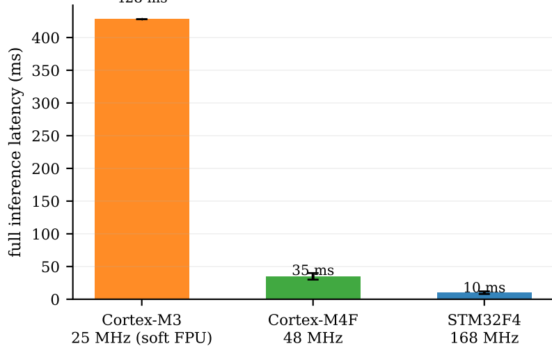
Projected MCU latency (2 GDN-2 layers, L=64)
