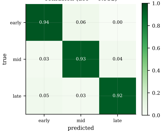
confusion (acc = 0.932)
