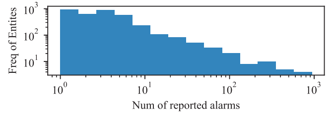
Fig. 2. Frequency distribution histogram of the number of alarms that one entity ever reported in the dataset.
