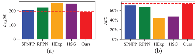
Fig. 5. NLLs and accuracies on a test dataset of various trained event models. (a) NLL. (b) Accuracy.
