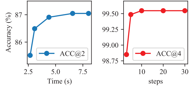
Fig. 6. Relationship between the time consumption and accuracy in RCA.
