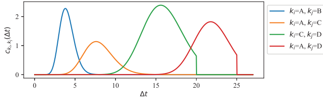
Fig. 3. Event intensity of each event type varies with the time difference \Delta t . The symbols in the parenthesis represent the causative event types.
