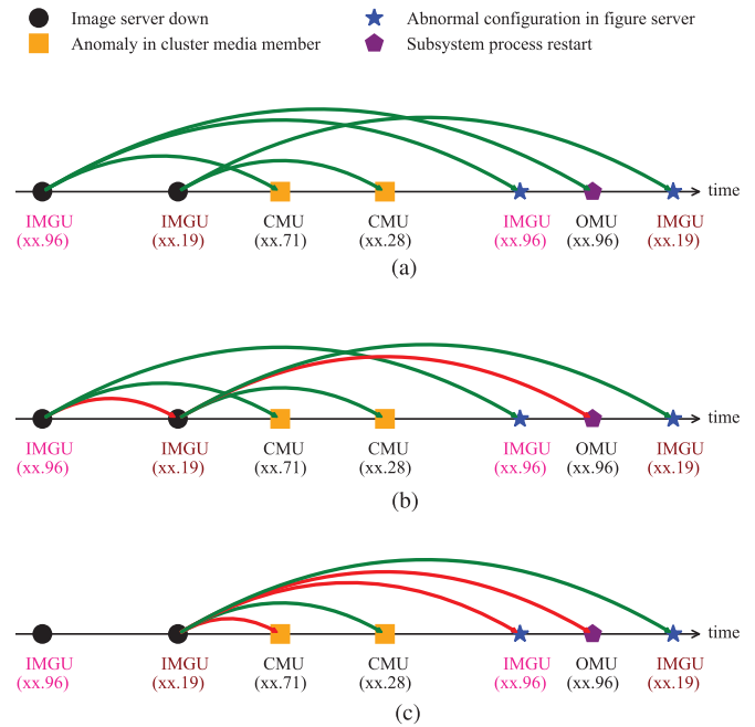
Fig. 7. Visualization of detected causative alarms compared with the ground truth. (a) Ground-truth causative alarms. (b) NEC (ours). (c) CAUSE.
