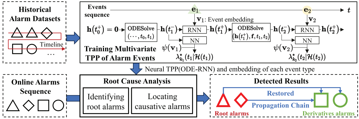
Fig. 1. Overall structure of NEC.
