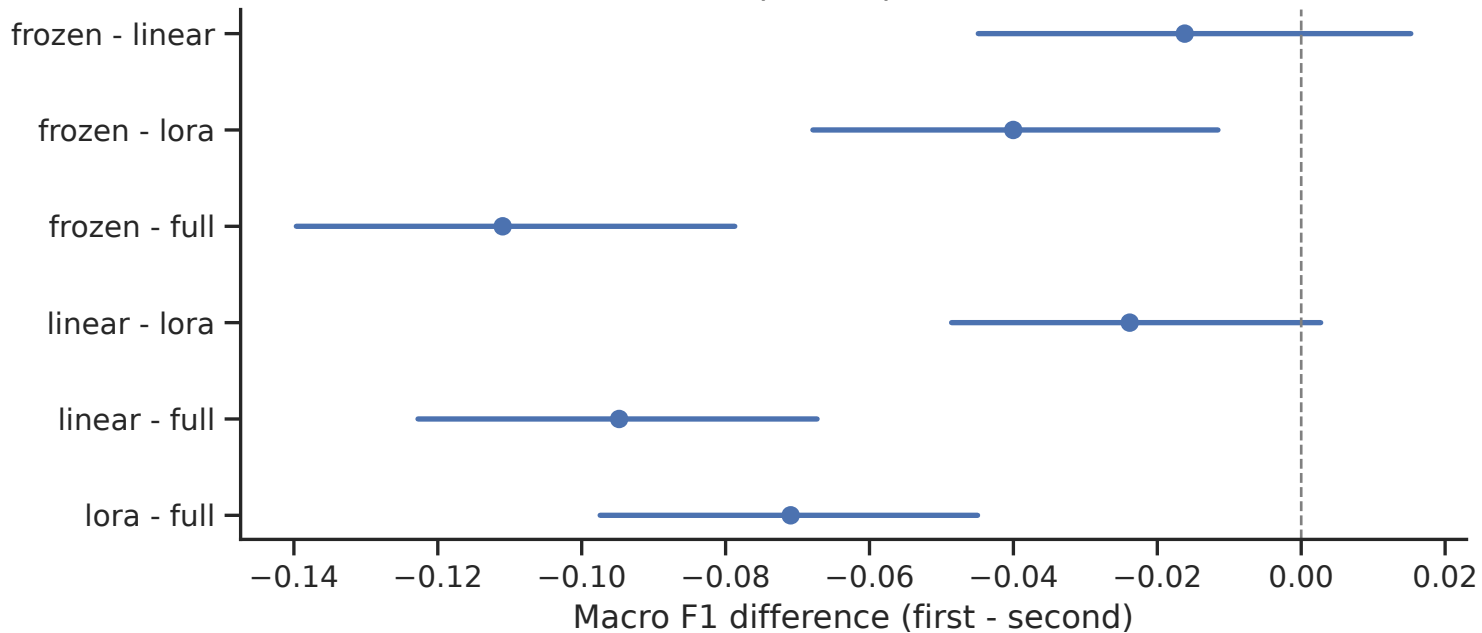
Paired bootstrap: 95% percentile intervals
