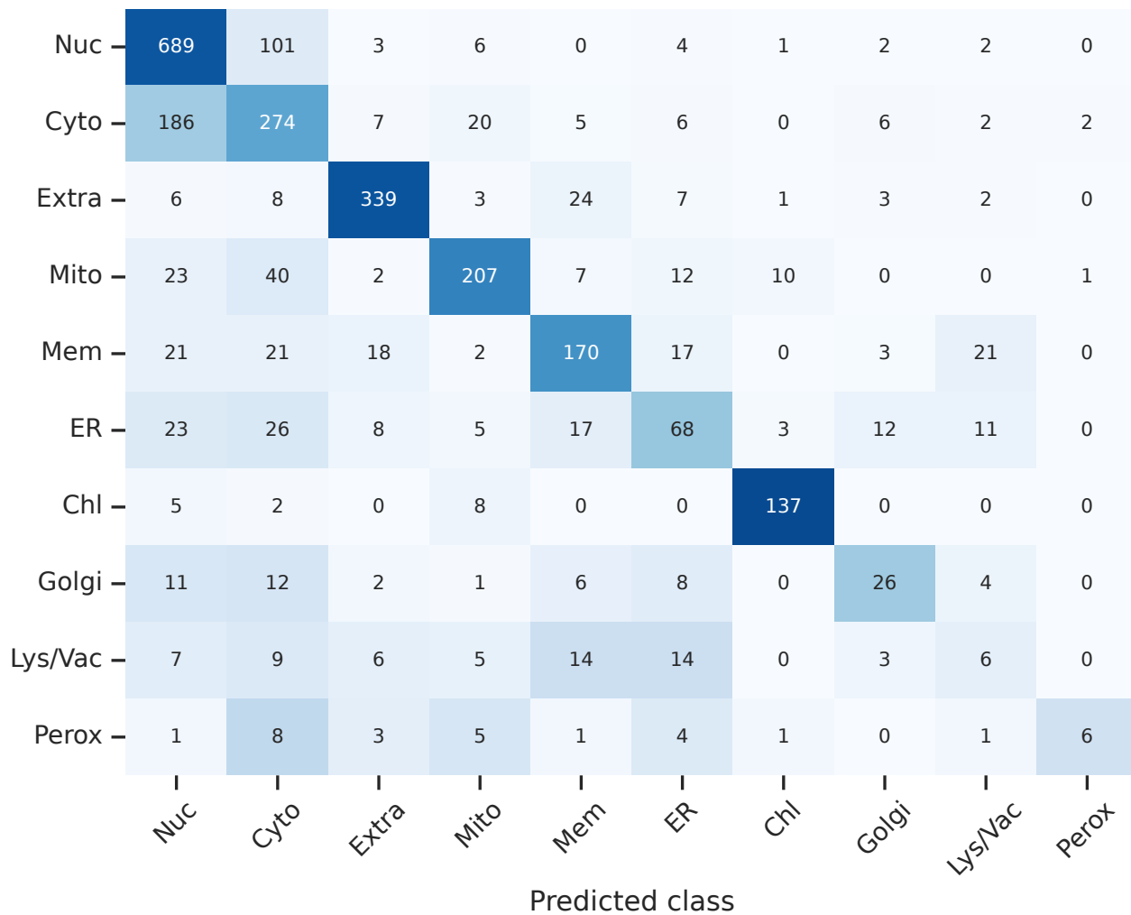
Frozen + kNN (counts; row-normalized color)
