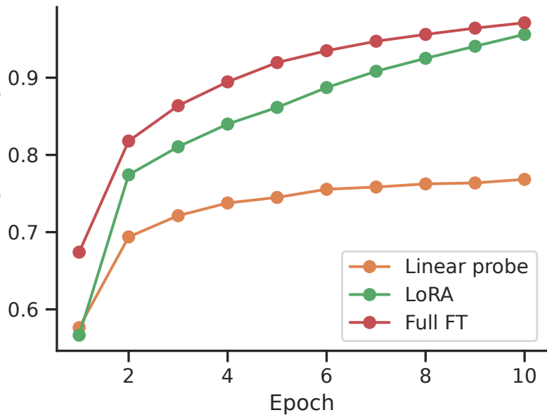
Training accuracy
