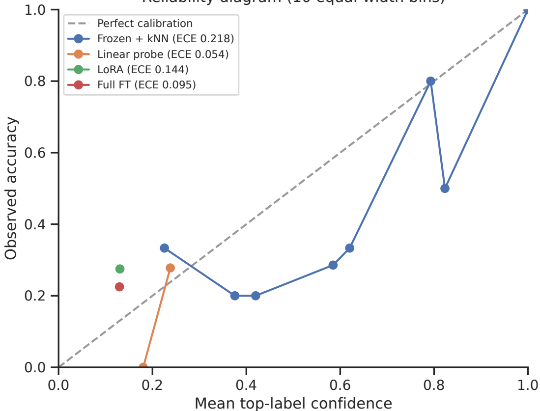
Reliability diagram (10 equal-width bins)
