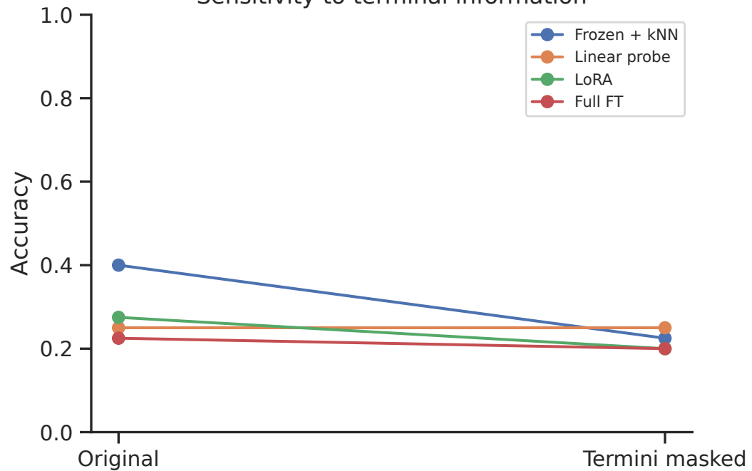
Sensitivity to terminal information
