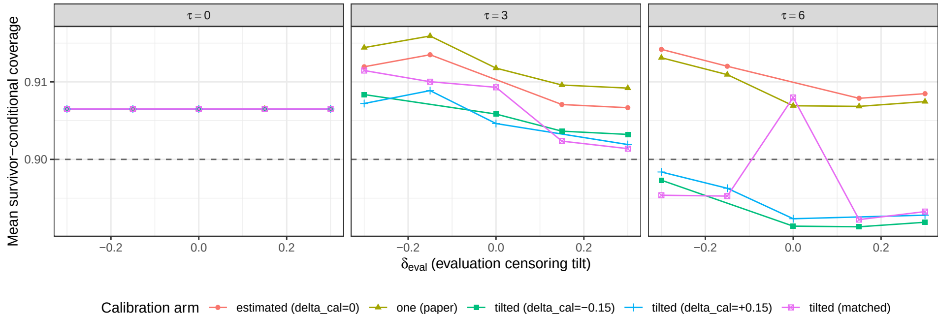
Censoring-shift sensitivity (linWB1, R=200, n=1000)
