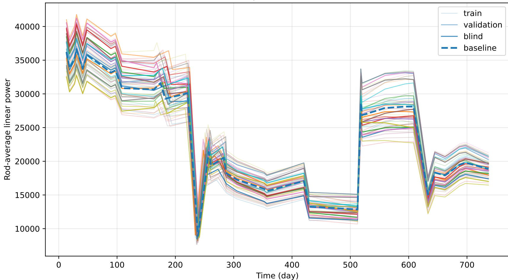
Generated variable power histories for POD--LSTM
