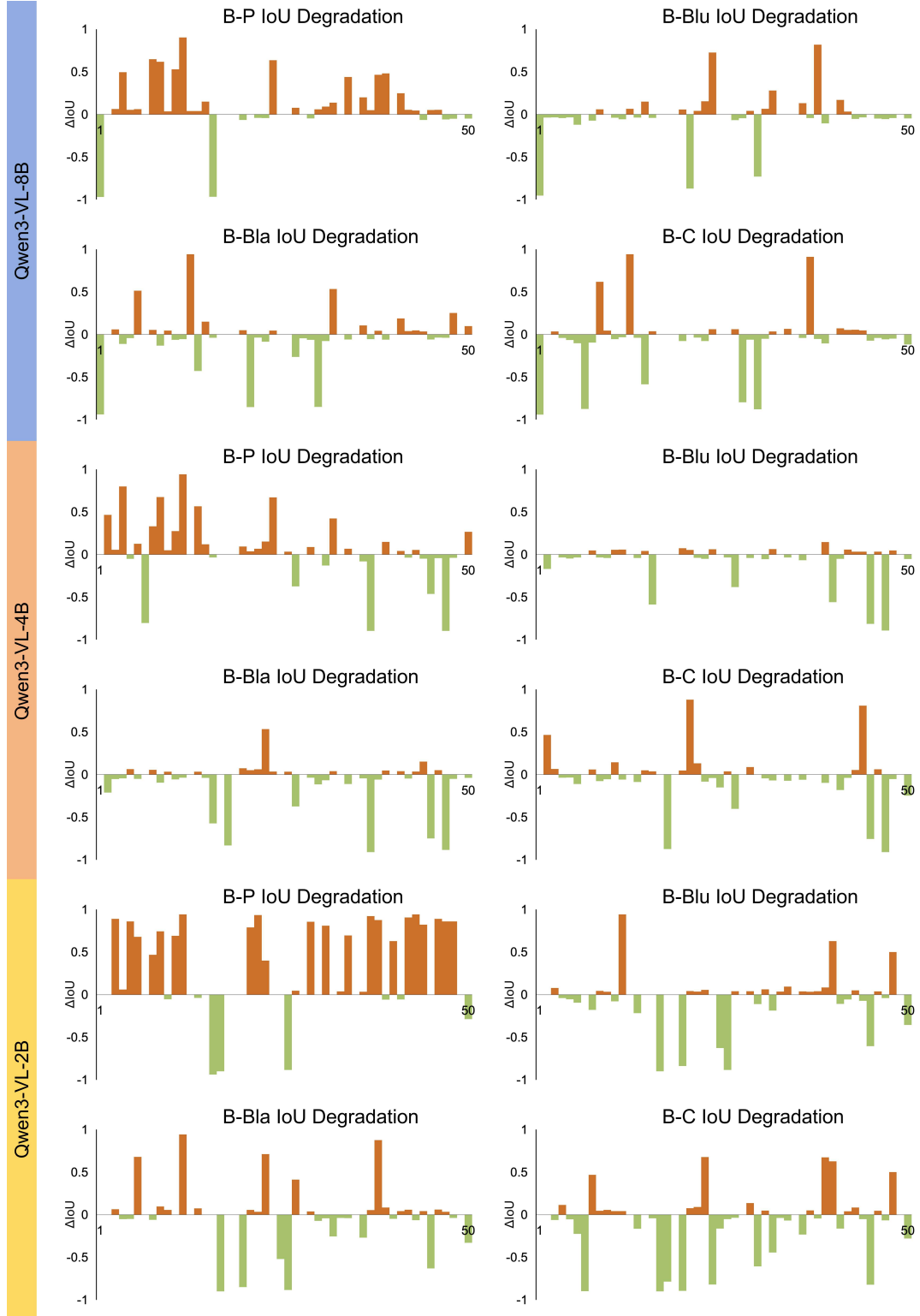
Figure 4: Detailed breakdown of per-method localisation accuracy across model scales.
