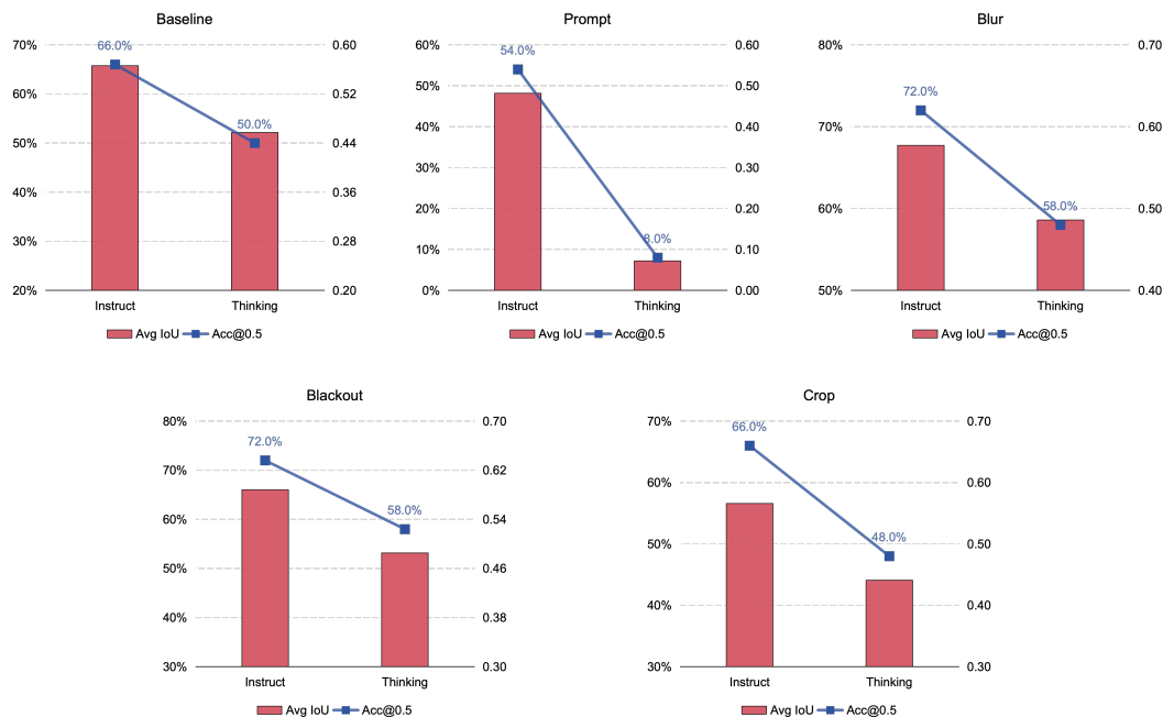
Figure 5: Comparison of Thinking and Instruct modes across the five attention-guiding methods.
