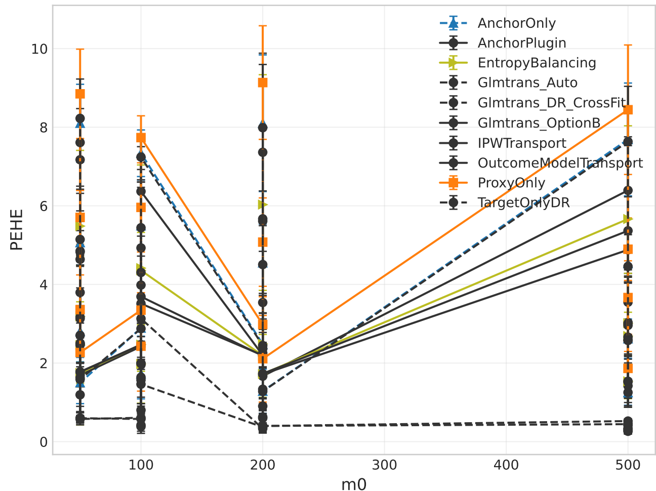
PEHE vs m_0 ( \downarrow lower is better)
