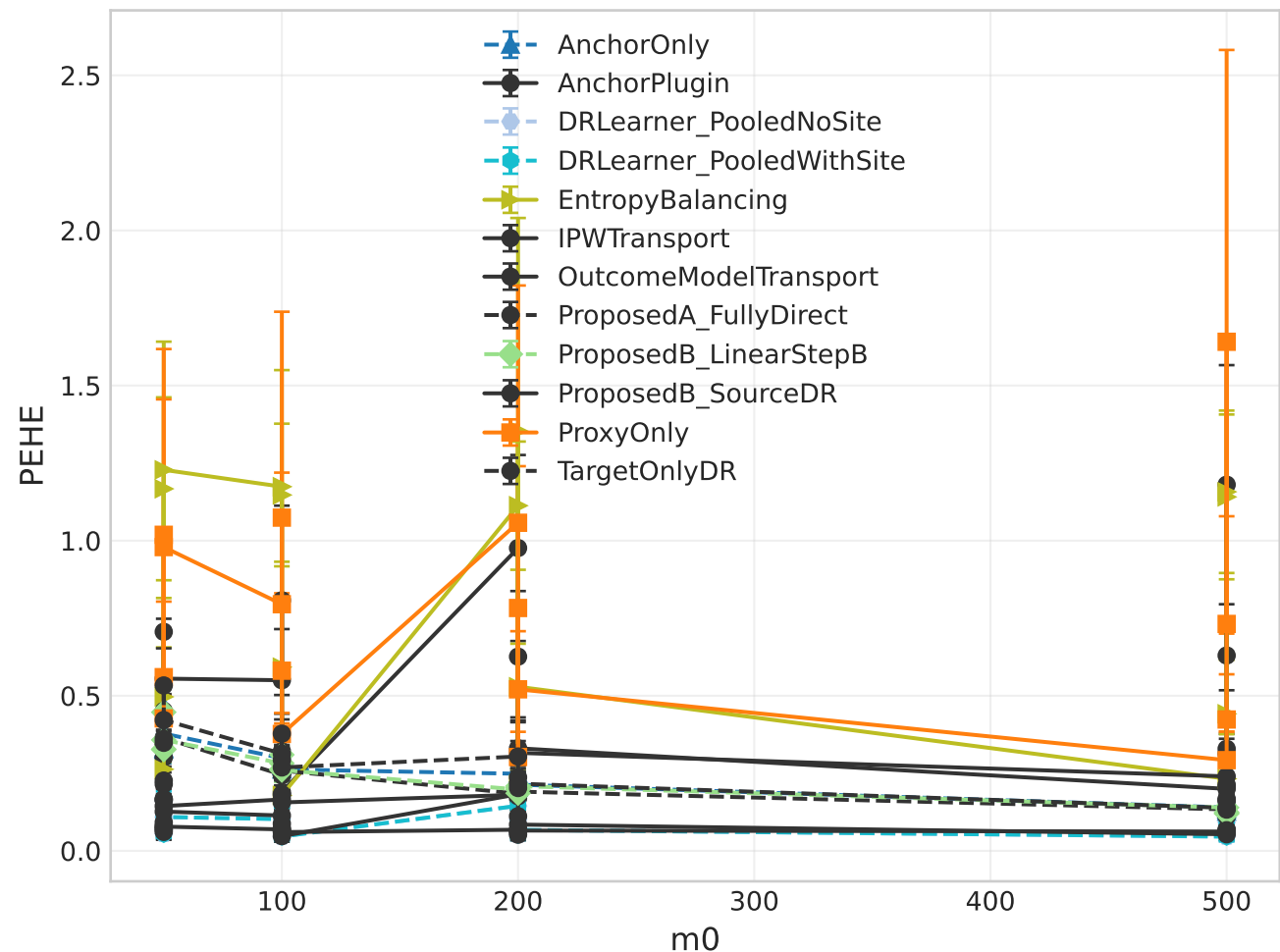
PEHE vs m0 (↓ lower is better)
