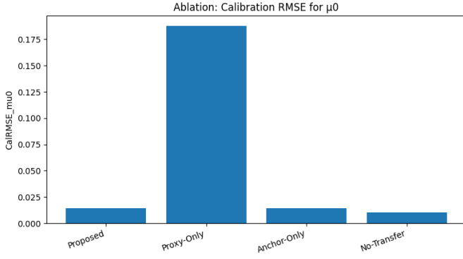
Fig. 3. Bar Plot of Calibration RMSE of placebo arms outcome of ablation study. Lower is better.
