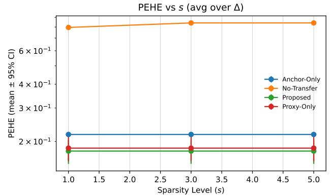
Fig. 8. PEHE vs. sparsity level s (mean \pm 95% CI), averaged over \Delta .
