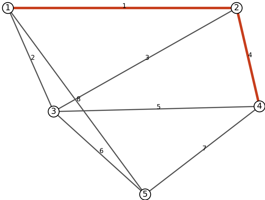
Figure 3 IEEE5 with mitigation
