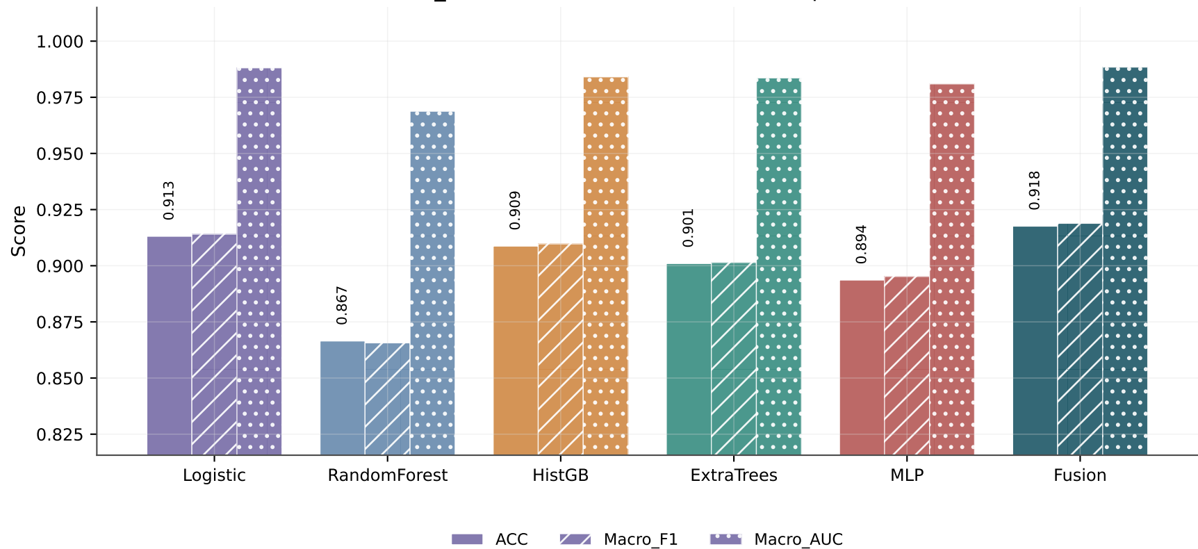
NO_DIRECT five-fold OOF model comparison
