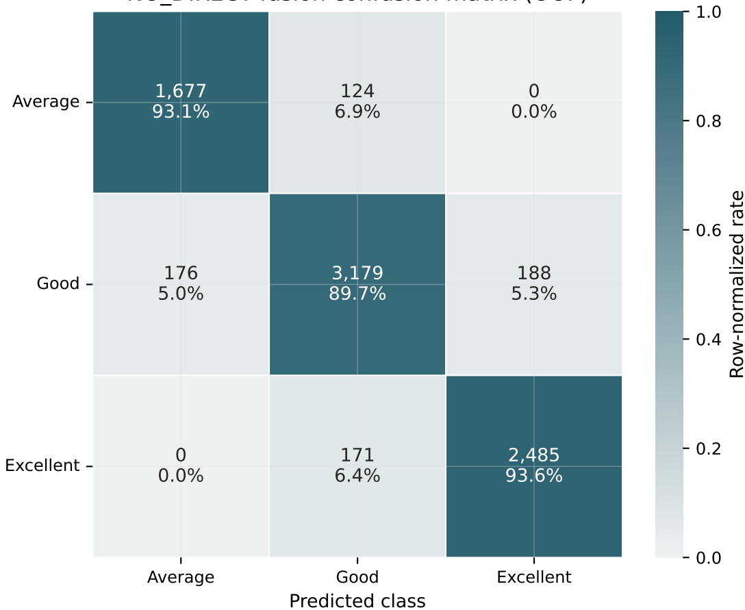
NO_DIRECT fusion confusion matrix (OOF)
