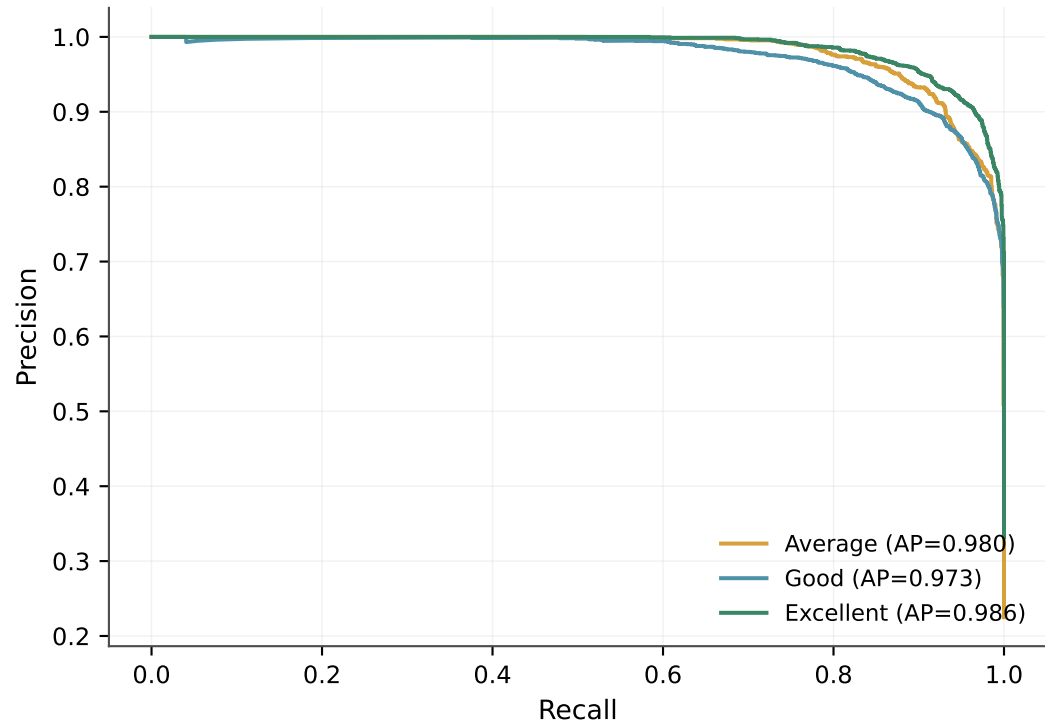
(b) One-vs-Rest PR
