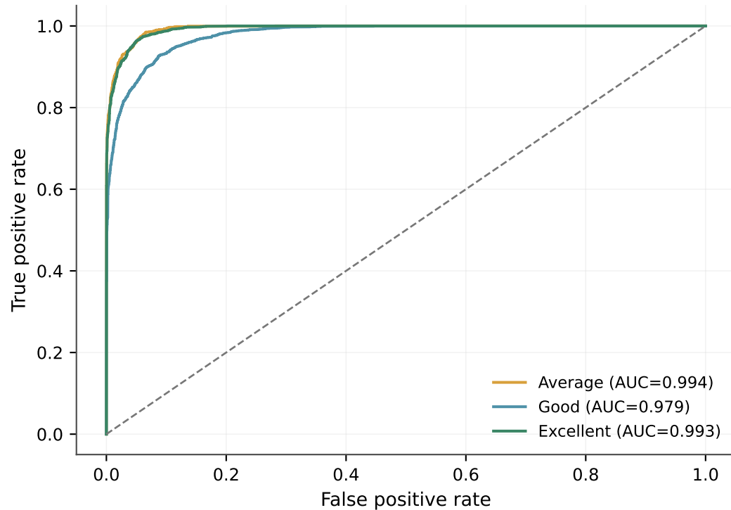
(a) One-vs-Rest ROC
