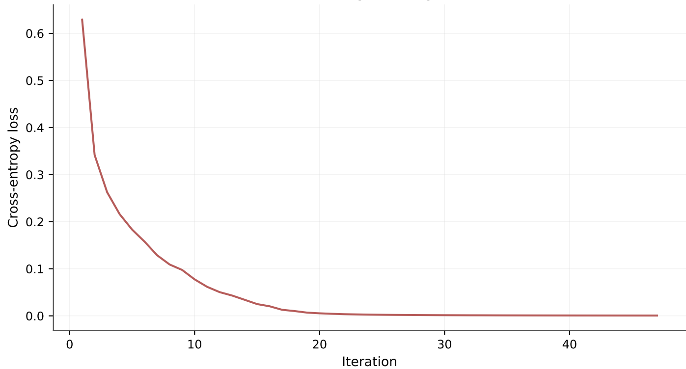
MLP training convergence
