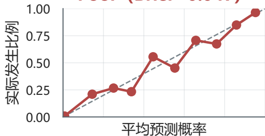
Good (Brier=0.106)
