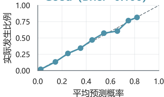
Good (Brier=0.106)
