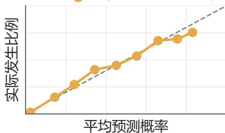
Average (Brier=0.105)
