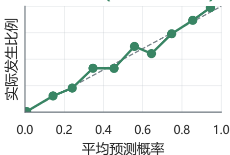
Excellent (Brier=0.047)
