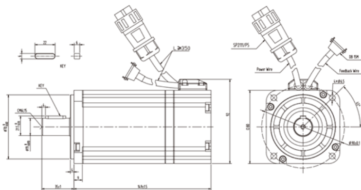
图 4-4 SMC80S-0040-30AoK-3DKH 伺服电机外形图
