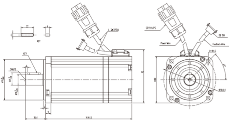
图 4-3 SMC80S-0040-30AoK-3DKH 伺服电机外形图
