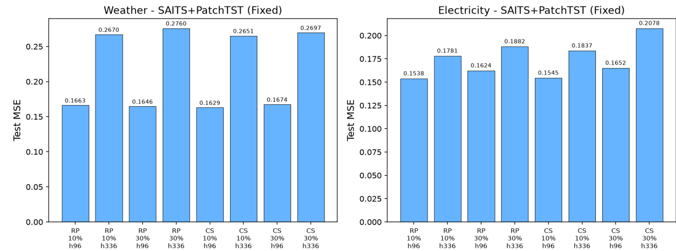
Group C: SAITS+PatchTST Overflow Fix Results
