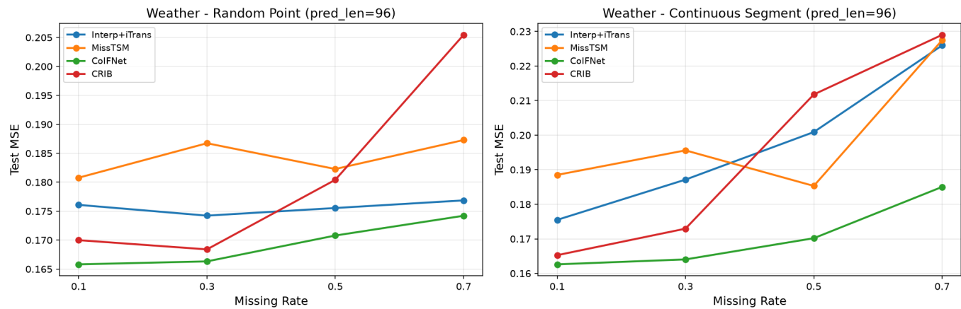
Missing Rate Trend: 10% → 70% (Weather)
