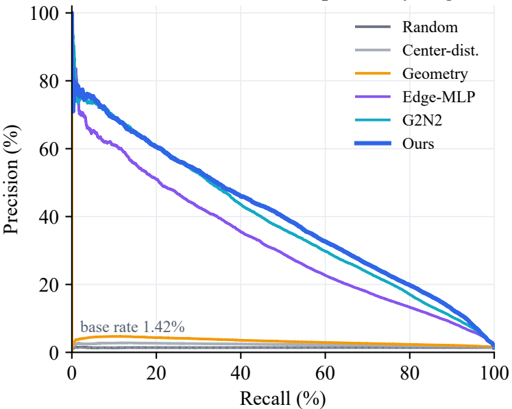
Precision–recall over dependency edges
