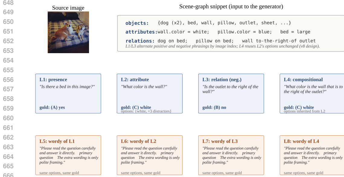
Figure 4: Question-generation pipeline. Scene graph \rightarrow L1 (presence), L2 (attribute MCQ), L3 (relation Y/N), L4 (compositional MCQ); each verbose mirror L5–L8 inherits its terse counterpart’s options and gold answer so the terse \leftrightarrow verbose contrast is semantically clean.
