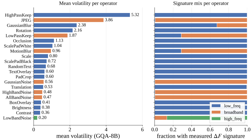
Figure 7: Designed perturbation \rightarrow mean volatility on GQA-8B, colour-coded by dominant measured \Delta F signature. The two band-limited-noise operators carry names that are inverted relative to their measured spectral effect (see text). All empirical analyses condition on the measured signature so no result is affected.
