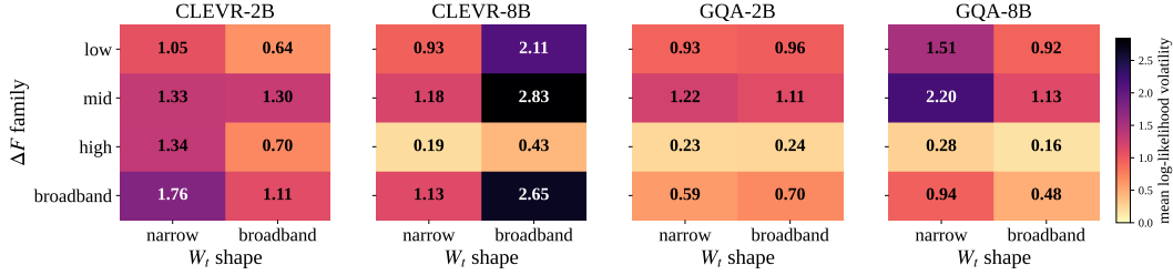
Figure 2: Mean log-likelihood volatility per (\Delta F, W_t(\omega)) cell, image-space last_2, all four runs. Narrow W_t(\omega) is higher than broadband in 4/4 rows on CLEVR-2B and GQA-8B. On CLEVR-8B all four rows reverse because broadband- W_t(\omega) cells there are overwhelmingly verbose mirrors near the log-prob ceiling, exhibiting large absolute swings from having more room to fall (the recovery-dominance regime of §3.5). On GQA-2B per-row differences are within \pm 0.11 (sampling noise). The mechanism reads: narrow W_t(\omega) amplifies drift on top of whatever ceiling-dynamics the model is in.
