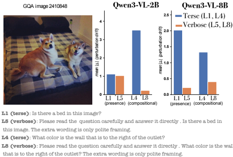
Figure 1: Verbose prompts improve VLM robustness On the same image and semantically identical questions, we show across 78 image corruptions and multiple VLMs, verbose paraphrases (L5, L8) significantly increase the mean log-likelihood of the correct answer (reducing uncertainty) for both a simple presence question (L1) and a hard compositional question (L4).
