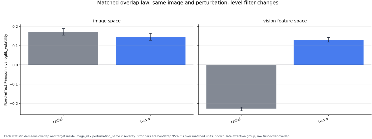
Figure 7: Matched-FE within-cell Pearson: image vs feature space, radial vs 2D. Within each (image \times perturbation \times severity) cell only the task level varies (L1–L8). Bars are the FE-Pearson correlation between within-cell demeaned overlap and within-cell demeaned log-likelihood volatility, with bootstrap 95% CIs. Left (image-space): both radial and 2D forms are positive and significant—the law works within-cell. Right (vision-feature space): the radial form is strongly negative, the 2D form is positive—the apparent “feature-space sign flip” is a radial-reduction artefact. The paper’s headline within-cell median Pearson ( r = 0.350 / 0.457 / 0.543 in Table 5.5) uses the stronger last_2 layer-group; this plot is the late third for which the matched-FE auxiliary script was run.
