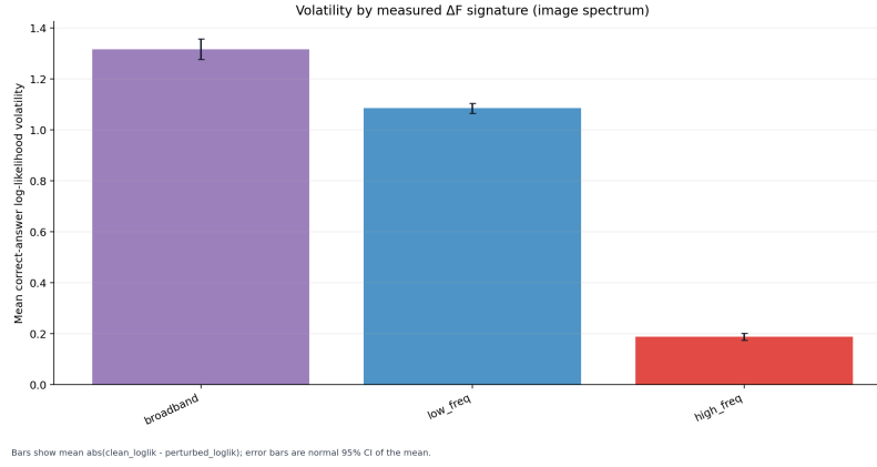
Figure 10: Mean log-likelihood volatility by measured \Delta F signature, marginalising over W_t(\omega) (100-sample 8B, image-space). Broadband perturbations are most damaging (mean 1.32, n = 14,384 ) because they overlap W_t(\omega) somewhere ; low-frequency perturbations land where W_t(\omega) does live and damage substantially (1.09, n = 45,976 ); high-frequency perturbations sit in the band where W_t(\omega)^{(\text{last\_2})} has thinned out, so they barely move the conditional likelihood (0.19, n = 2,040 ). 95% CIs on the mean.
