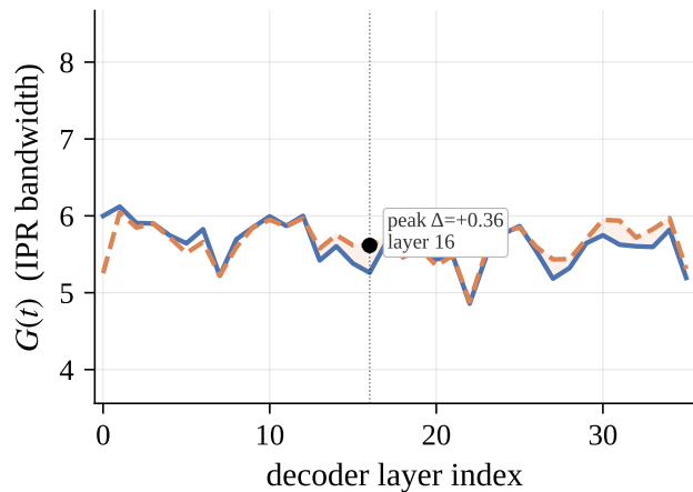
GQA-8B (B=7)
