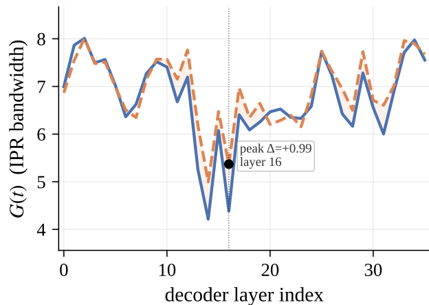
CLEVR-8B (B=9)
