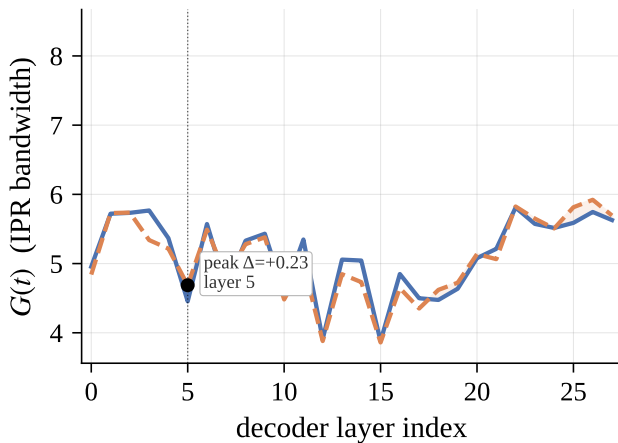
GQA-2B (B=7)
