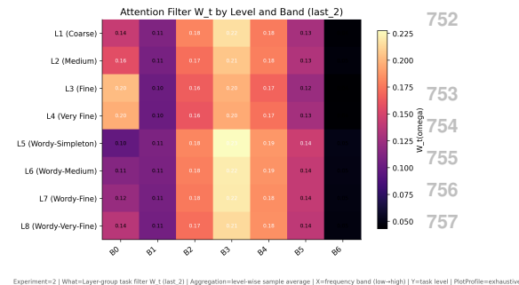
Figure 6: Cross-modal attention spectrum W_t(\omega) across L1–L8 at B = 7 bins. Primaries (top) concentrate mass downward as C_{\text{sem}} rises; wordy mirrors (bottom) keep a broader distribution.
