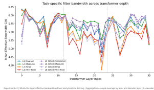
Figure 2: Layer-resolved bandwidth G(t) across all 36 decoder attention layers (8B, 100 samples). Solid: primaries L1–L4. Dashed: wordy mirrors L5–L8. Vertical dashed lines mark layer-group thirds. The four stages of the trajectory are visible: a sharp layer-0 length prior (wordy below primary by −0.74), erasure by layer 2, length-insensitive content narrowing through mid, and a re-opened wordy-broader gap peaking at +0.33 at layer 31.
