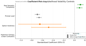
Figure 1: Forest plot of the tug-of-war (100-sample 8B, primary target log-likelihood volatility). Pooled OLS (circles) and within-image fixed effects (squares) both give \hat{\beta}(C_{\text{res}}) > 0 (destabilises) and \hat{\beta}(C_{\text{prompt}}) < 0 (stabilises). 1000-image 2B run gives larger magnitudes (+0.29/−0.32, R^2 = 0.22 , p < 10^{-130} / p < 10^{-209} ).
