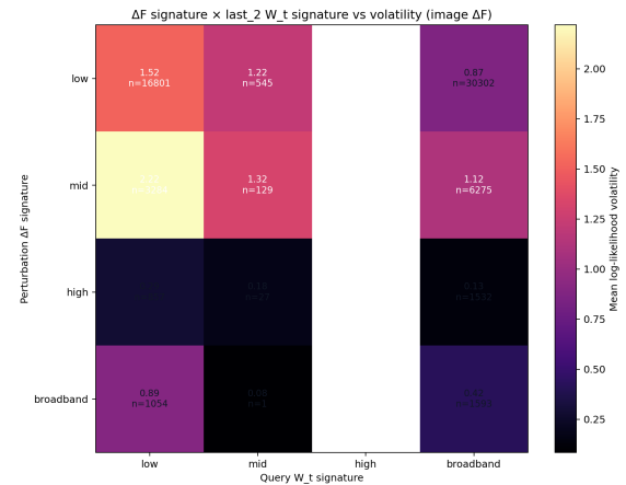
Signatures use low/mid/high mass fractions plus normalized entropy. Correlations use W_t \Delta F vs \text{abs}(\loglik\_drift) inside each cell.
