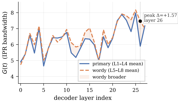
GQA-2B (B=7)
