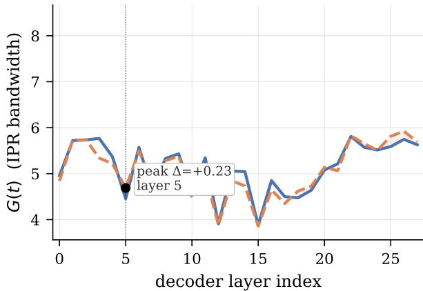
GQA-2B (B=7)
