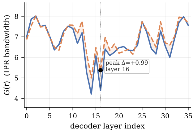
GQA-8B (B=7)
