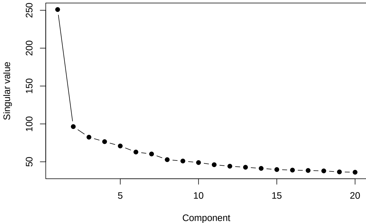
Singular-value spectrum of the cleaned bipartite network
