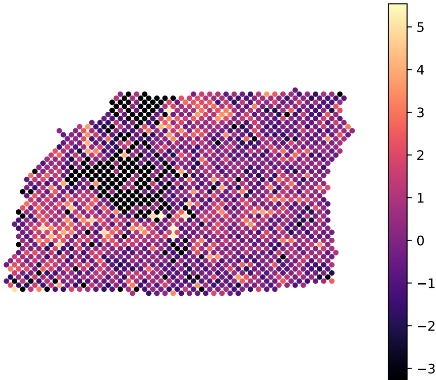
GSM6177618 SPP1_myeloid_score
