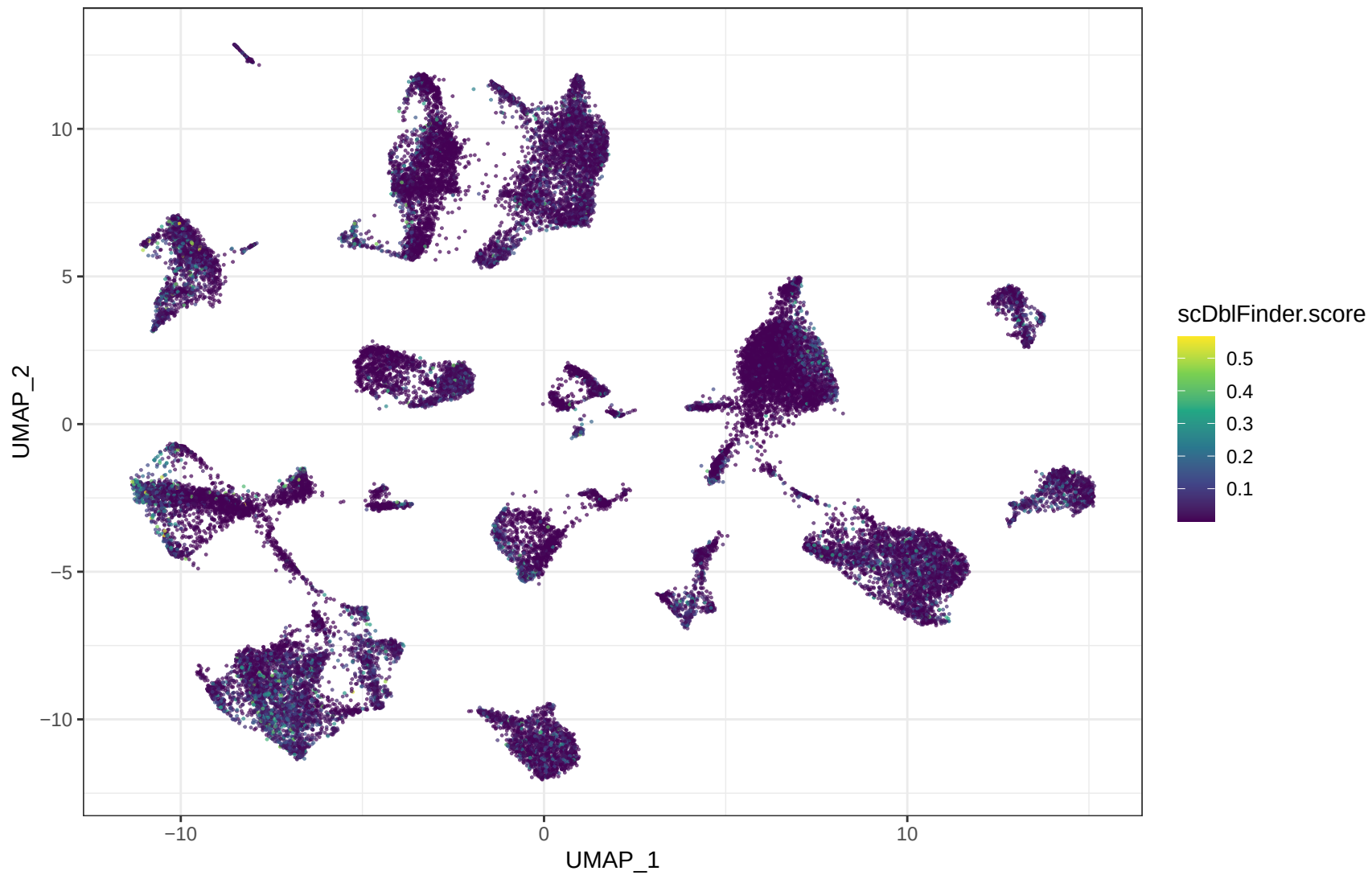
GSE154600 UMAP_by_doublet_score
