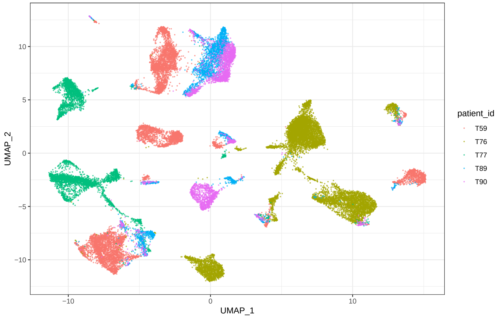
GSE154600 UMAP_by_patient
