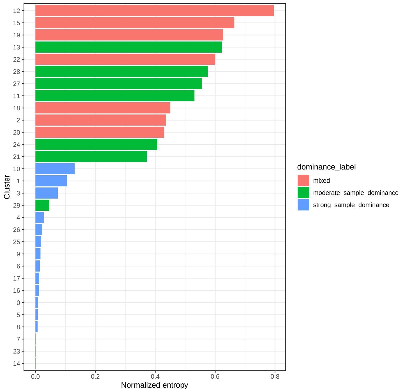
GSE154600 cluster sample entropy
