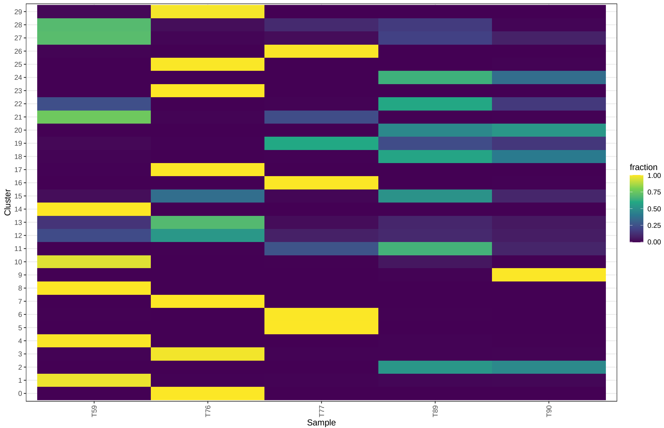
GSE154600 cluster sample fractions
