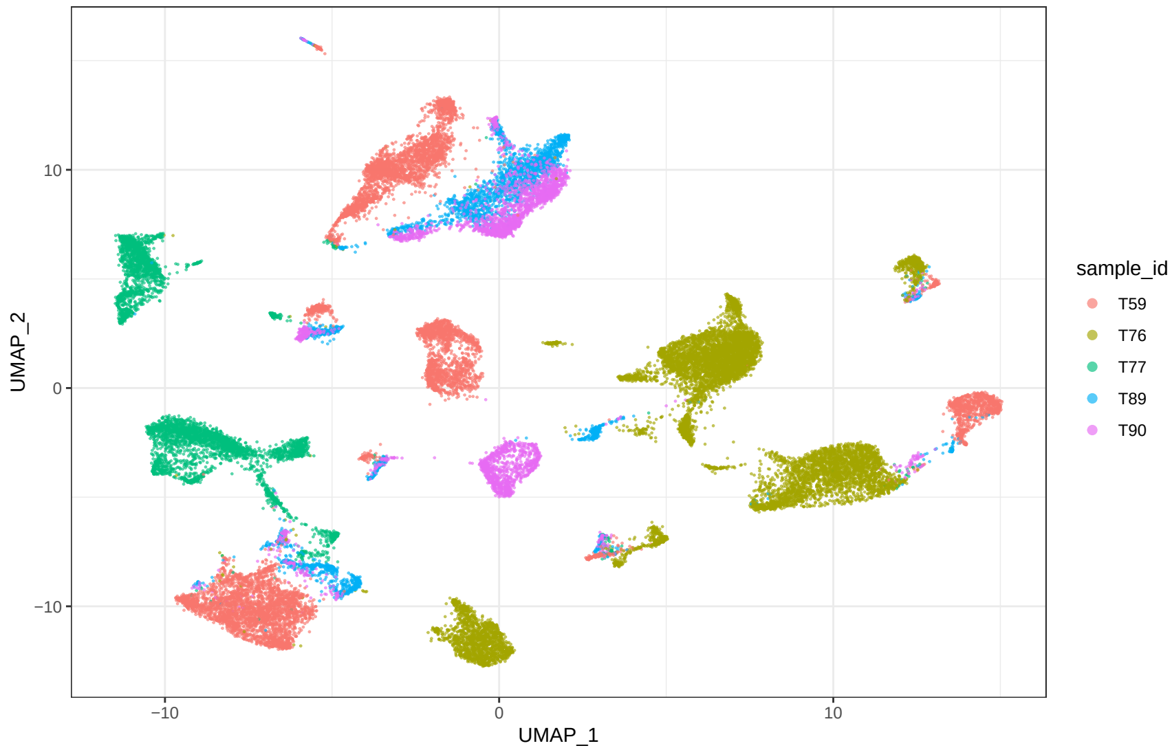
GSE154600 Combined_broad_lineages A_uncorrected samples
