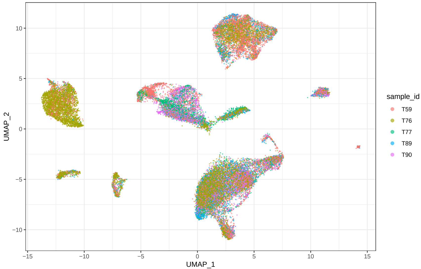
GSE154600 Combined_broad_lineages B_harmony_sample samples
