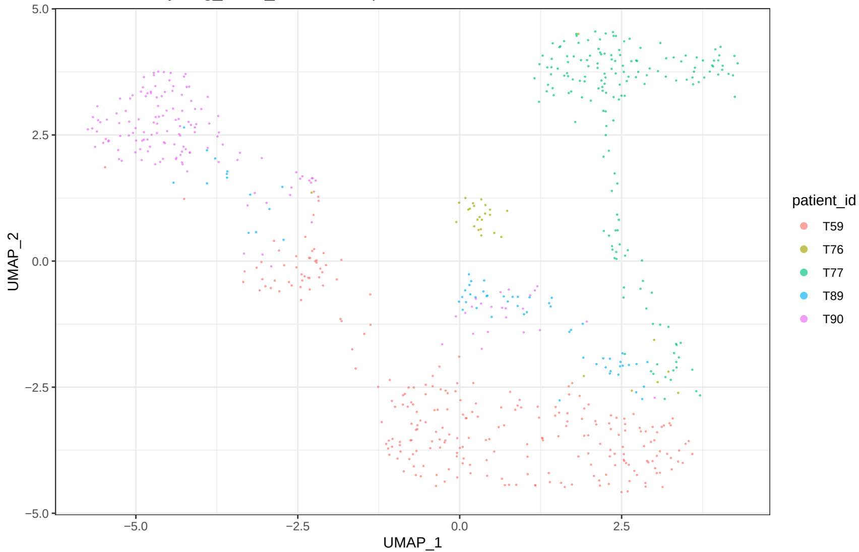
GSE154600 Cycling_like A_uncorrected patients
