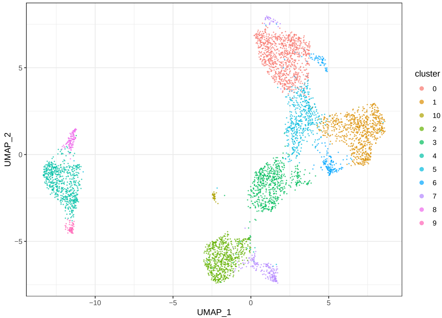
GSE154600 Epithelial_like B_harmony_sample clusters
