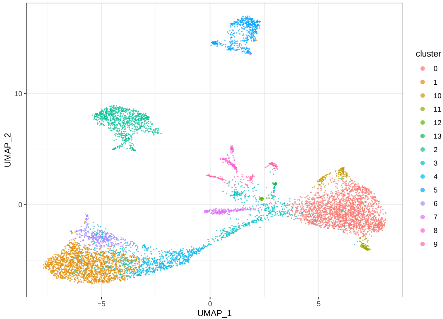
GSE154600 Fibroblast_like A_uncorrected clusters
